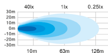
Flood Beam
