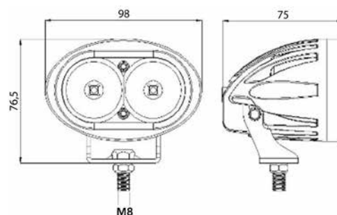
30° Spot Light
