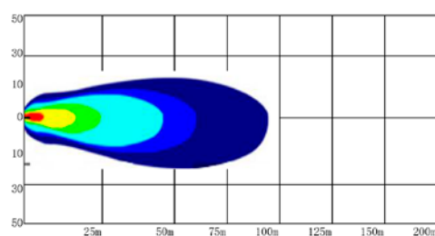
30° Spot Light
