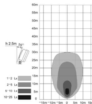
Flood beam KW-242F
