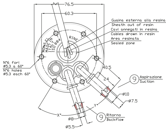
FLANGIA: VISTA "B" FLANGE: "B" VIEW
