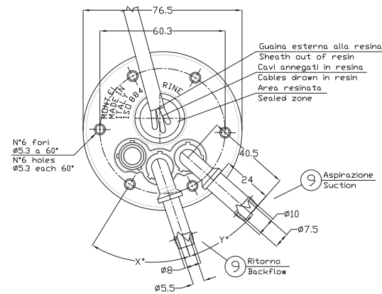
FLANGIA: VISTA "B" FLANGE: "B" VIEW
